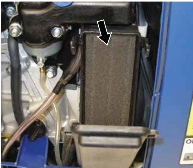
Figure 32 – Foam Element (WH1000i Shown)
